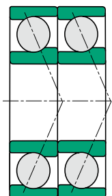
DT arrangement (tandem)
