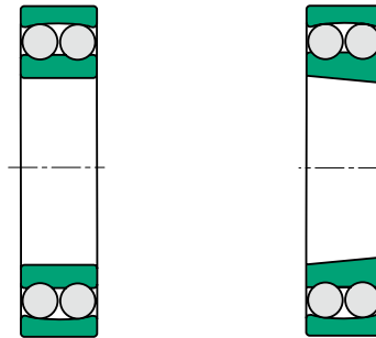
Cylindrical Bore
