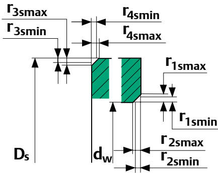
Tapered roller bearings dimensions in inches and mm
