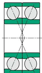
DF arrangement (face to face)
